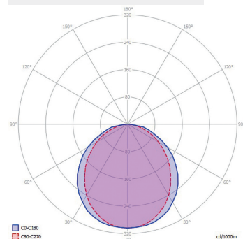
Polar Diagram
